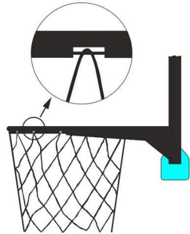
Diagram 5 Attachment of the net (example)
